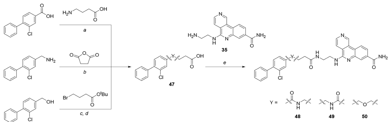
Scheme 7. Synthesis of Compounds 48–50, Incorporating Alternatives to the Benzylic Amine a
