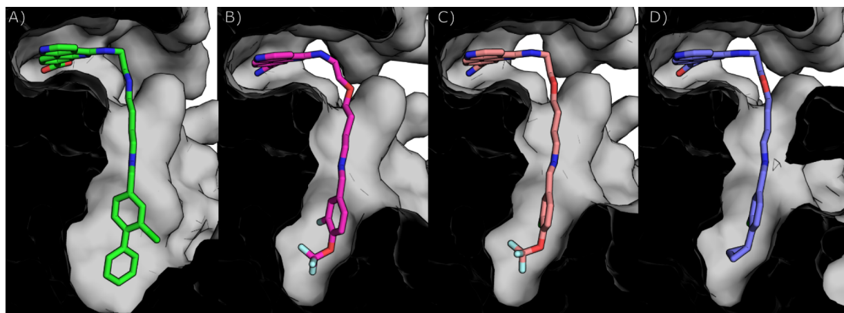
Figure 4. Crystal structures of compounds binding in the \alpha D pocket. Cross-section of the binding modes of: A) 18 (green); B) 54f (pink, PDB: 7I84); C) 54e (salmon pink, PDB: 7I89); D) 54b (purple, PDB: 7I8B).
