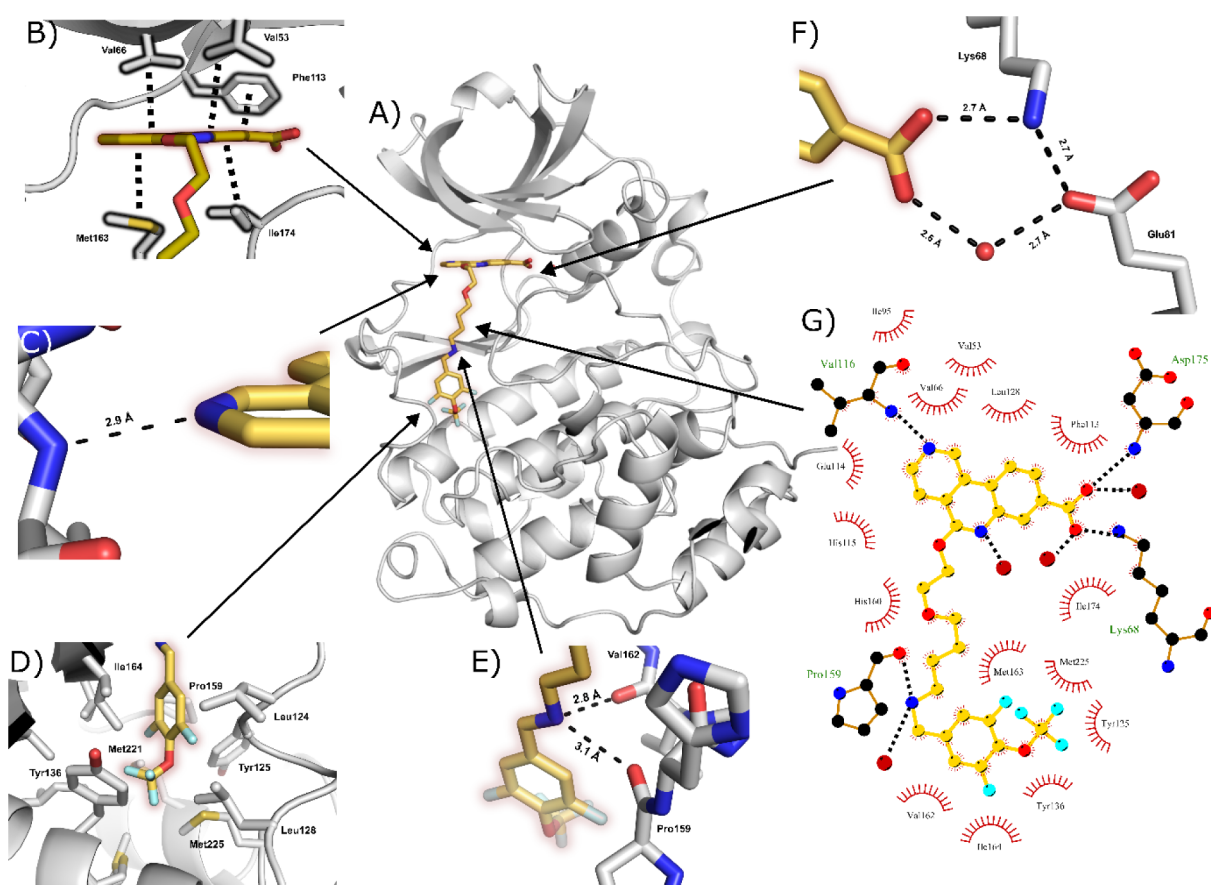
Figure 6. Binding mode of 61f to CK2 \alpha . A) The crystal structure of 61f bound to CK2 \alpha (PDB: 7I8K). B) The interactions of 61f within the ATP-binding site. C) The hydrogen bonding interactions between 61f and the hinge region. D) The hydrophobic interactions between 61f and the \alpha D pocket. E) The hydrogen bonds between the benzylamine and CK2 \alpha . F) The hydrogen bonding network between the carboxylic acid group of 61f , Lys68, Glu81 and a water molecule. G) Two-dimensional map of the interactions between CK2 \alpha and 61f (gold) with hydrogen bonds shown as dotted lines, and hydrophobic interactions depicted with spiked arcs (or “eyelashes”).
