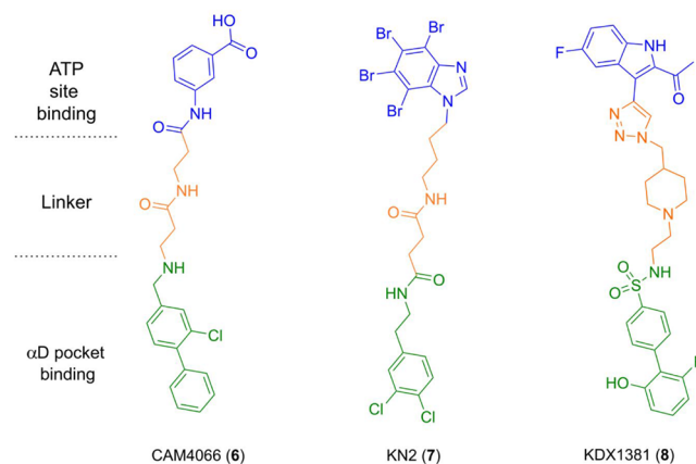
Chart 2. Chemical Structures of Selected Bivalent CK2 \alpha Inhibitors
