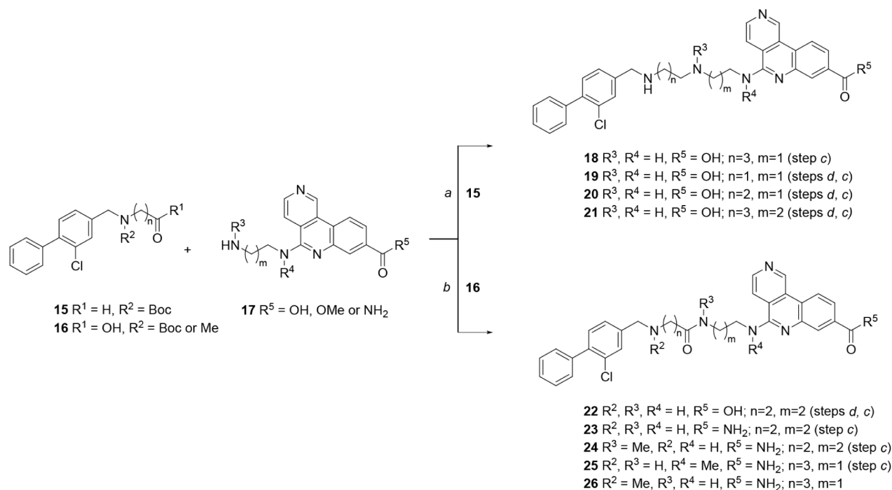
Scheme 3. General Synthetic Routes to Compounds 18–26, Incorporating Initial Changes to the Linker a
