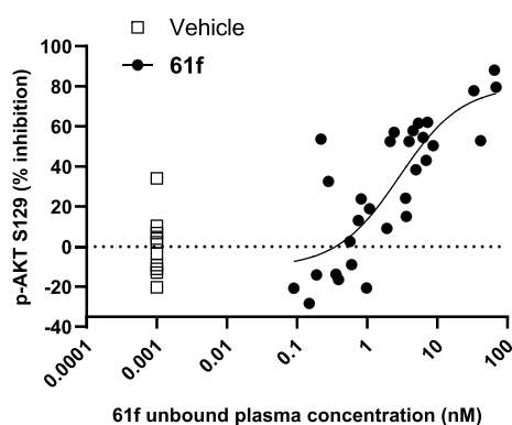
Figure 8. In vivo inhibition of p-AKT S129 in HCT116-tumors in mice following oral administration of 61f. Concentration–response curve for p-AKT S129 inhibition in tumor was generated using the unbound concentration of 61f in plasma from all individual mice in each dose group (10, 30, 100 mg/kg) at either 2 or 8 h postfinal dose, and the corresponding p-AKT S129 measurement from tumor tissue determined by Western blotting.
