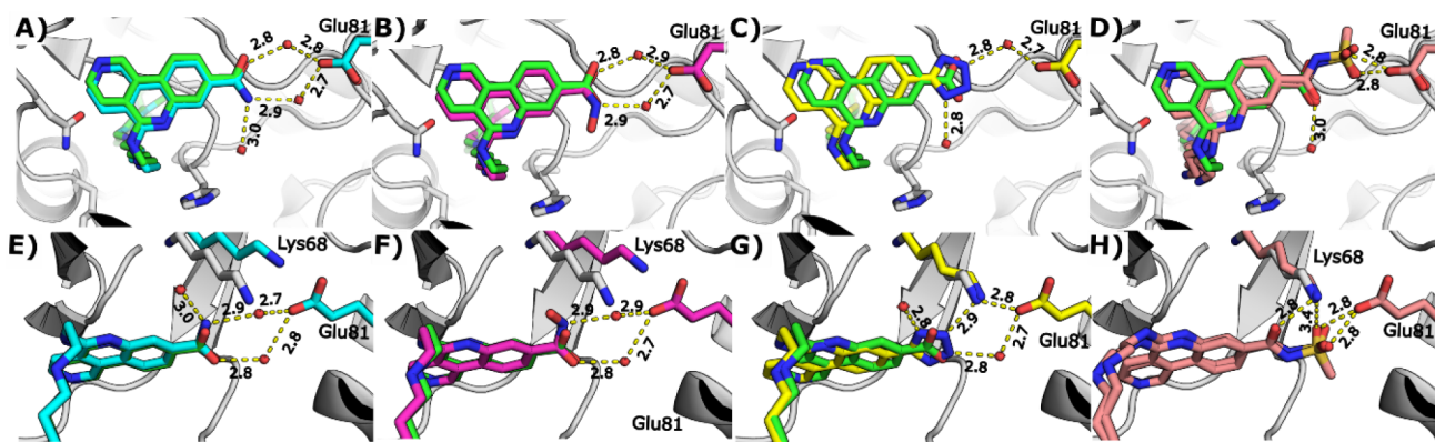
Figure 2. Crystal structures of compounds that show the hydrogen bonding networks of carboxylic acid isosteres. A) and E) The binding mode of 30 (blue, PDB: 7I7Y) compared to 18 (green). B) and F) The binding mode of 31 (pink, PDB: 7I7Z) compared to 18 (green). C) and G) The binding mode of 33 (yellow, PDB: 7I83) compared to 18 (green). D) and H) The binding mode of 32 (salmon pink, PDB: 7I84) compared to 18 (green). Hydrogen bonds are shown as dotted lines.
