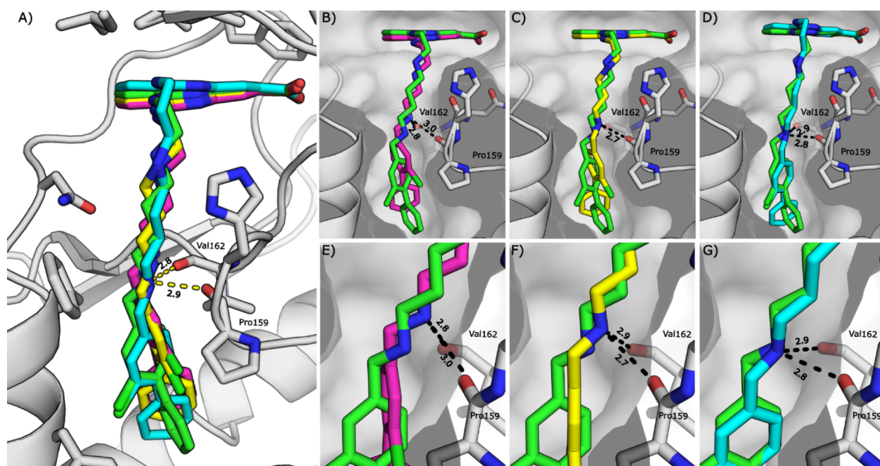
Figure 3. Crystal structures showing compounds with various linker lengths. A) The binding mode of 18 (green) compared to 19 (pink, PDB: 7I80), 20 (yellow, PDB: 7I82) and 21 (blue, PDB: 7I8P). Hydrogen bonds between 18 and Val162 and Pro159 are shown as dotted lines. B) and E) The binding mode of 18 (green) compared to 19 (pink). Hydrogen bonds between 19 and Val162 and Pro159 are shown as dotted lines. C) and F) The binding mode of 18 (green) compared to 20 (yellow). Hydrogen bonds between 20 and Val162 and Pro159 are shown as dotted lines. D) and G) The binding mode of 18 (green) compared to 21 (blue). Hydrogen bonds between 21 and Val162 and Pro159 are shown as dotted lines.
