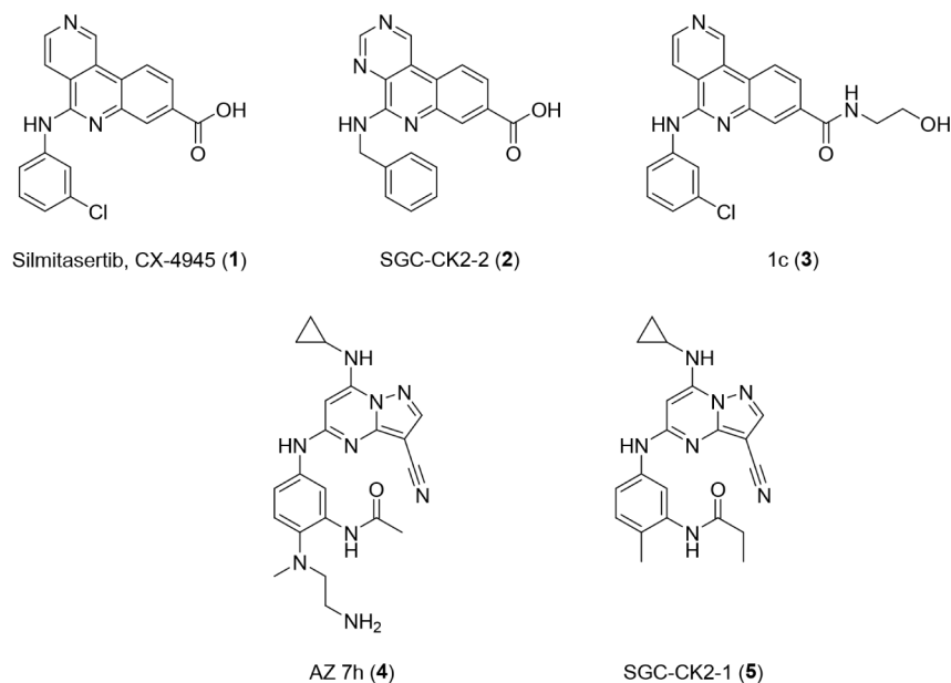
Chart 1. Chemical Structures of Selected Type 1 CK2 \alpha Inhibitors
