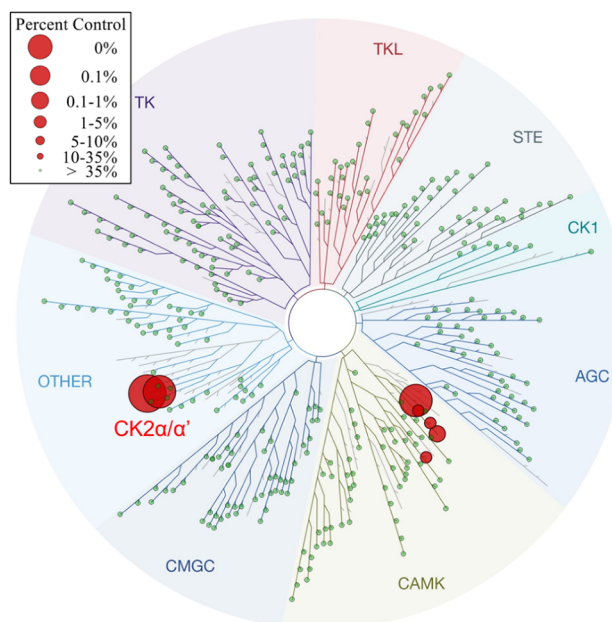
Figure 7. Profile of 61f in the KINOMEScan™ scanMAX panel. The human kinome is represented as a phylogenetic tree. Each kinase is shown as a sphere with size and color indicating the level of inhibition of each kinase at 100 nM APL-5125, as per legend on the top left corner.
