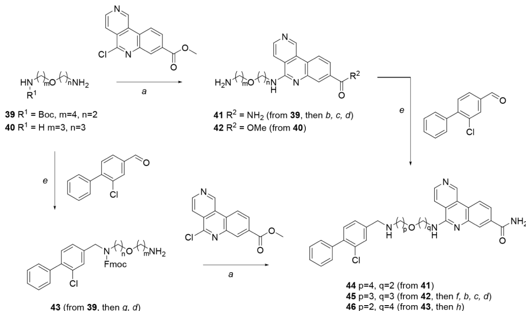
Scheme 6. Synthesis of Compounds 44–46, Containing an Ether Linker a
